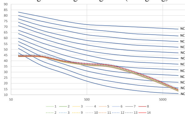
Figure 4. RC (16Hz-4000Hz).
