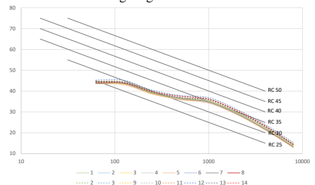
Figure 5. NC (63Hz-8000Hz).
