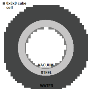
Figure 4. Spherical target within a spherical domain
