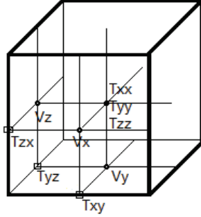
Figure 1. Computing stencil.
