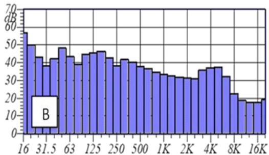
Frequency, Hz
