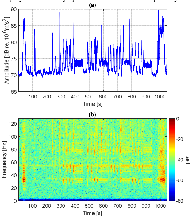
Figure 3. Time evolution of the 1-second moving average of the acceleration signal measured on the ground floor (a) and associated spectrogram (b).
