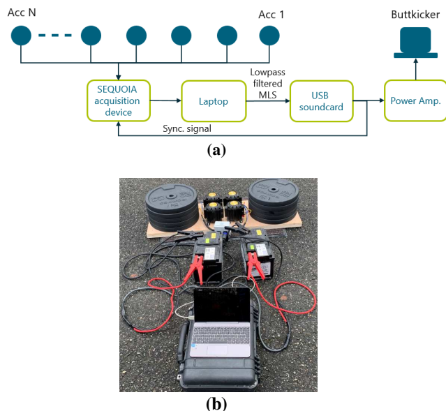
Figure 1. Schematic of the measurement system (a) and a photograph of the developed system (b).
