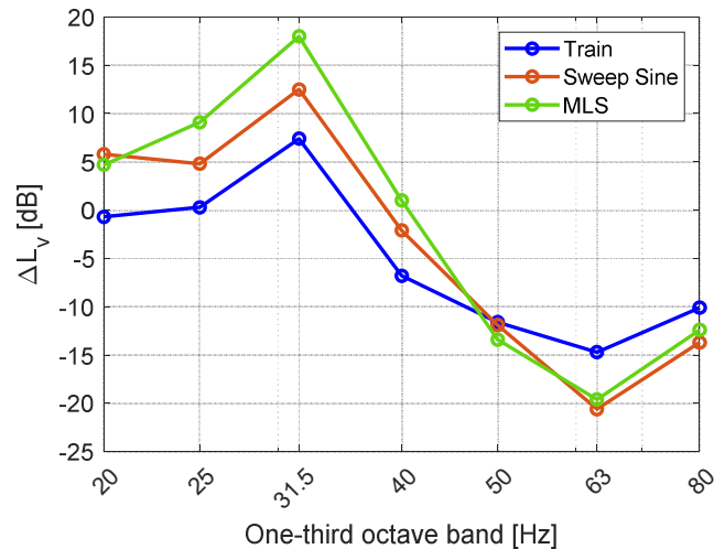
Figure 6. Ground to floor transfer function for the building calculated from Sweep Sine, MLS and train pass-by measurements.
