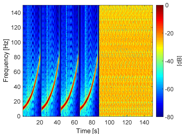
Figure 2. Spectrogram of the source signal of the measurement system.
