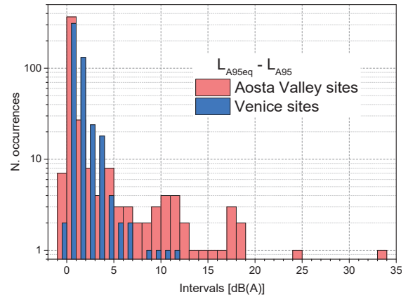
Figure 3. Histogram of the L_{A95eq} - L_{A95} differences.
