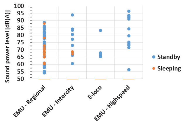
Figure 2. Sound power level of HVAC components.
