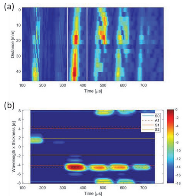
Figure 2. (a) Experimental B-Scan – (b) 2D-STFT of the experimental B-Scan
