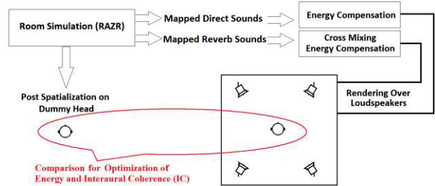
Figure 1. The perceptually-based audio reproduction system: The outputs of RAZR for direct and reverb parts of simulated RIRs are perceptually compensated and rendered over four loudspeakers in a reverb room. The dummy head in the reproduction room is compared with the simulated post spatialized dummy head in RAZR to obtain the compensation filters considering the energy and the interaural coherence (IC) criteria.
