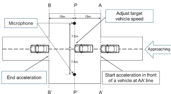
Figure 4. Layout for pass-by noise measurements
