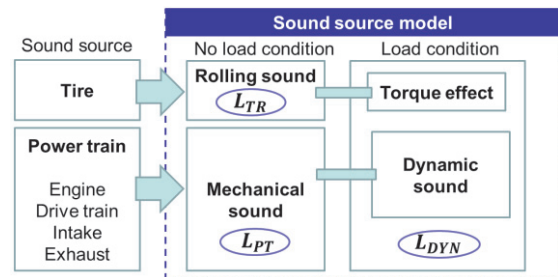
Figure 3. Structure for sound source model
