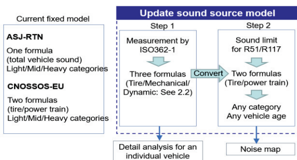
Figure 2. Concept for update of sound source model
