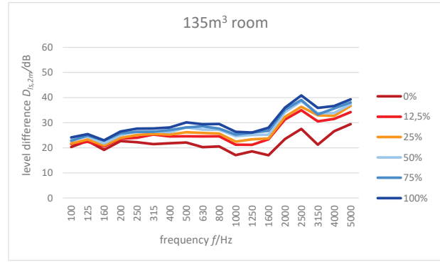
Figure 11. Level difference D_{ls,2m} for 135m 3 room at the variation of the surface of the panels.
