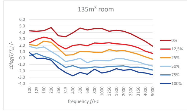
Figure 12. Correction term 10lg T/T_0 for 135m 3 room at the variation of the surface of the panels.
