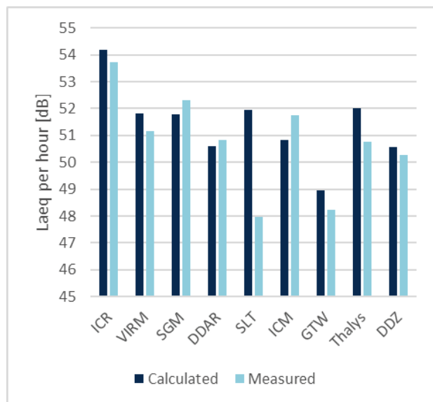
Figure 4. Comparison of calculated and measured immission values for different train types.
