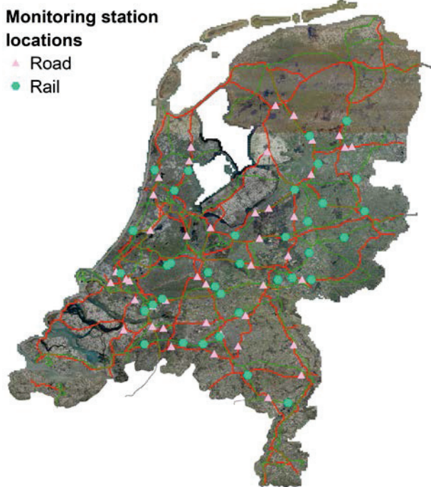
Figure 1. Location of noise monitoring stations along highways and railroads in the Netherlands.
