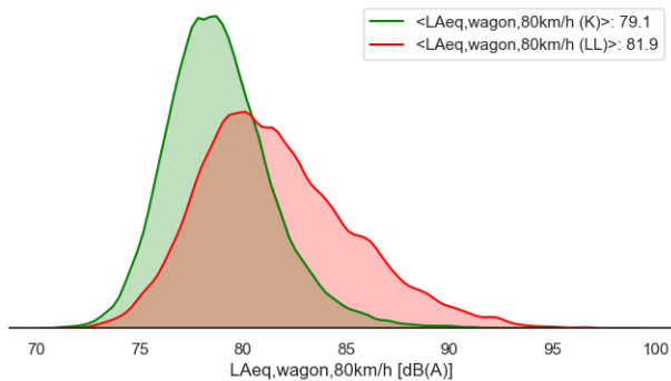
Figure 8. Density distributions of the L_{Aeq,80km/h} from 40k freight wagon labelled K and 13k labelled LL.
