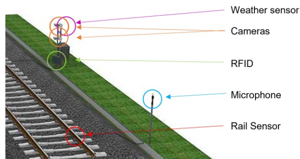
Figure 1. Schematic drawing of the setup with its key components.
