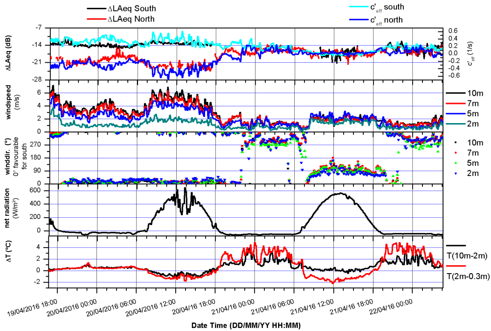
Figure 2: Sound level difference ( \Delta L_{A,eq,200m} = L_{A,eq,200m} - L_{A,eq,34m} ) and the effective sound speed gradient on both sides of the motorway in Bad Vöslau with meteorological data [4]
