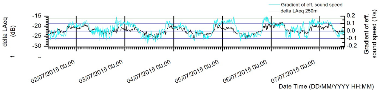
Figure 1: A good correlation between A-weighted sound level difference \Delta L_{Aeq, 250m} = L_{A,eq, 250m} - L_{A,eq, 18m} and the effective sound speed gradient (one week of the measurement period) is present
