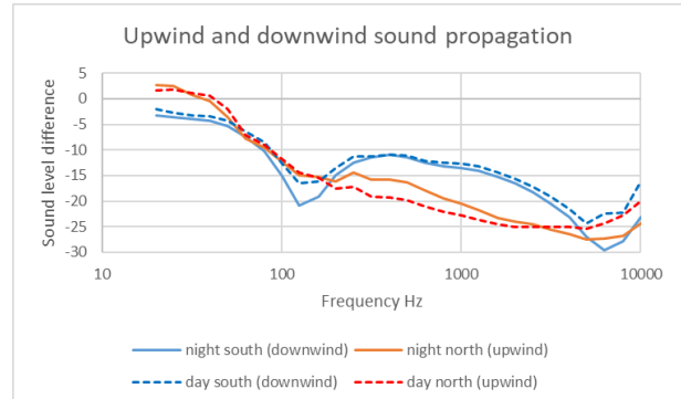
Figure 4: Frequency dependent sound level difference between up- and downwind sound propagation at Bad Voelslau
