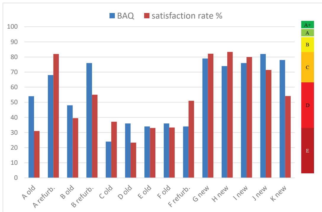
Figure 1. BAQ index for the investigated buildings.
