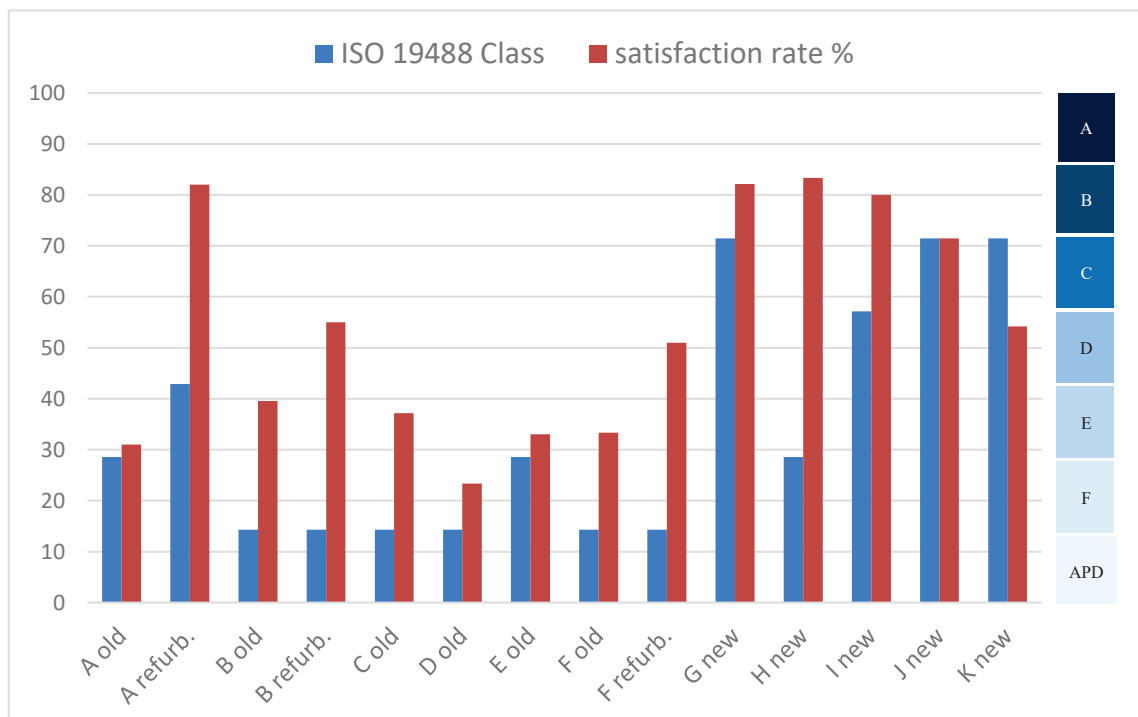
Figure 2. ISO/TS 19488 class for the investigated buildings.
