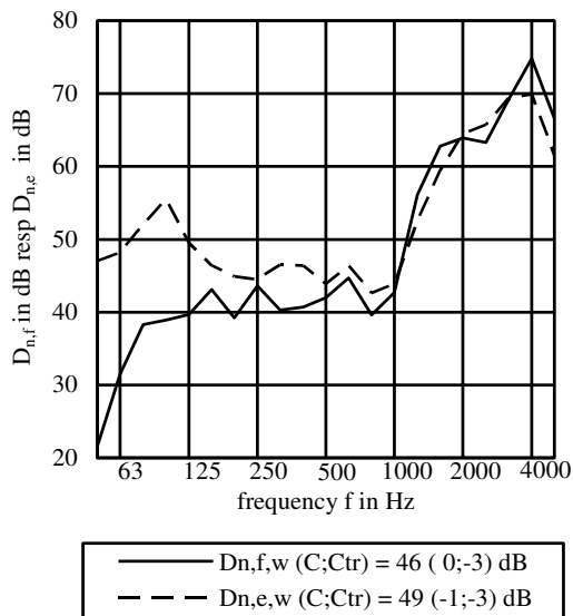
Figure 3 profile sound insulation and flanking sound insulation of a façade element, same profile of a element façade system, depth of Profile150 mm.
